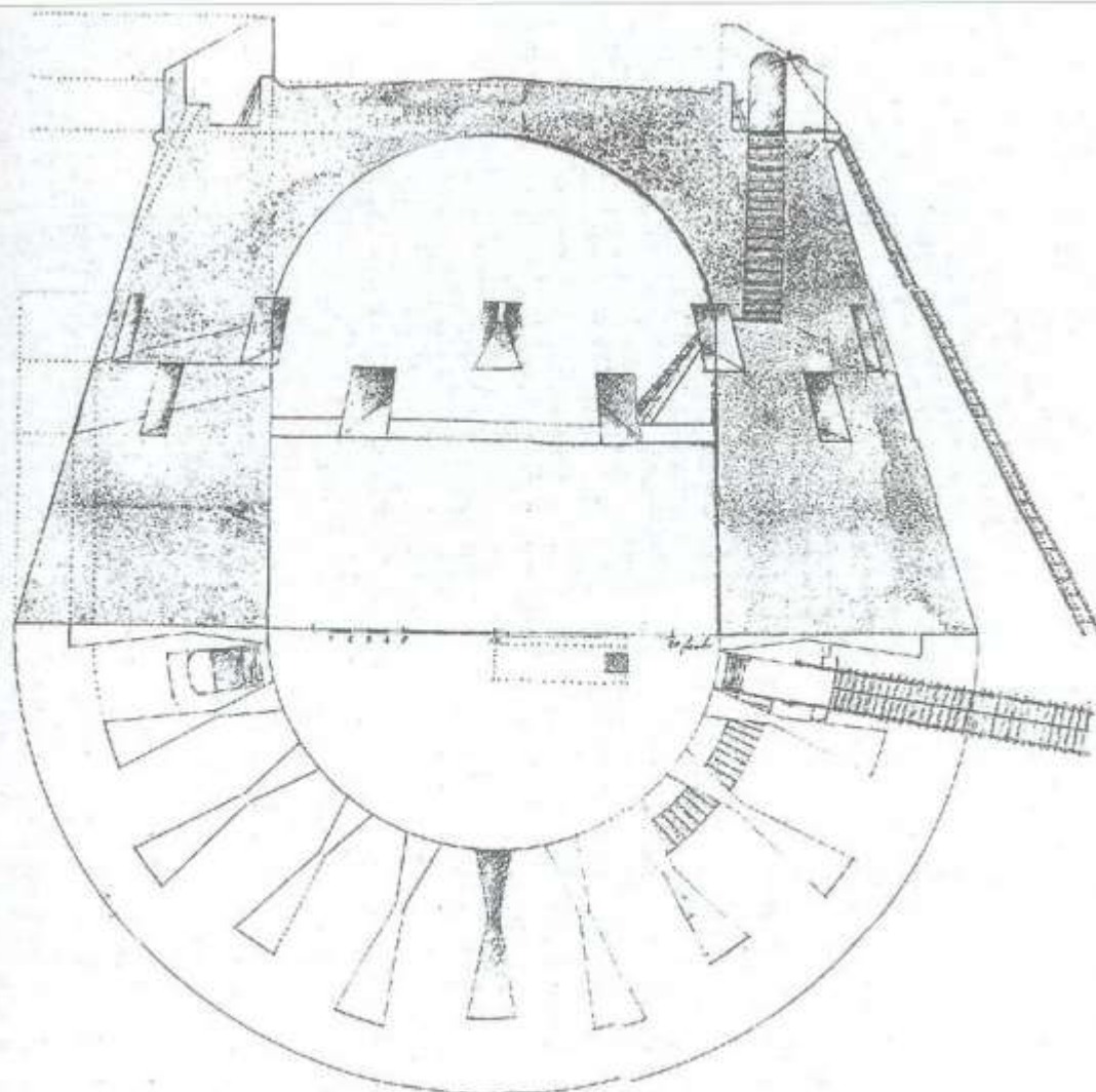
A Plan of Tower - Corzola , prepared by Captain B. W. Taylor R.A. and Lieut. J. Colclough, 81 st Regiment, February 1873.
